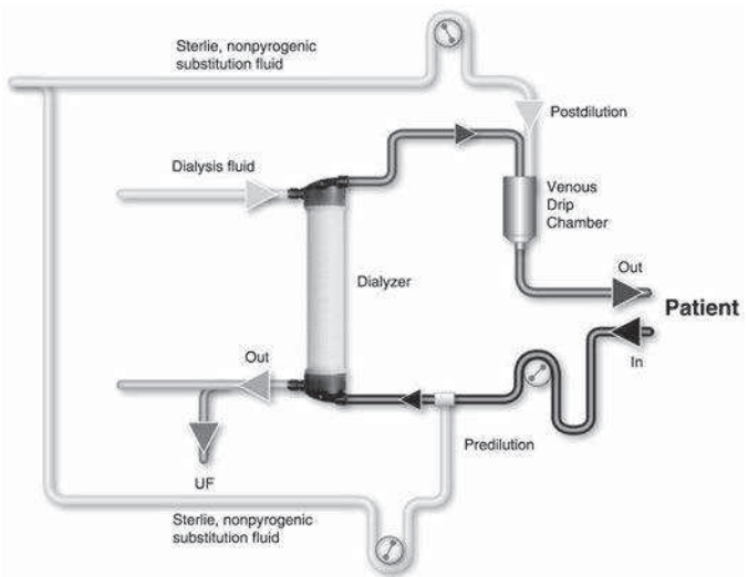
FIGURE 17.3 Mixed-dilution online hemodiafiltration.
