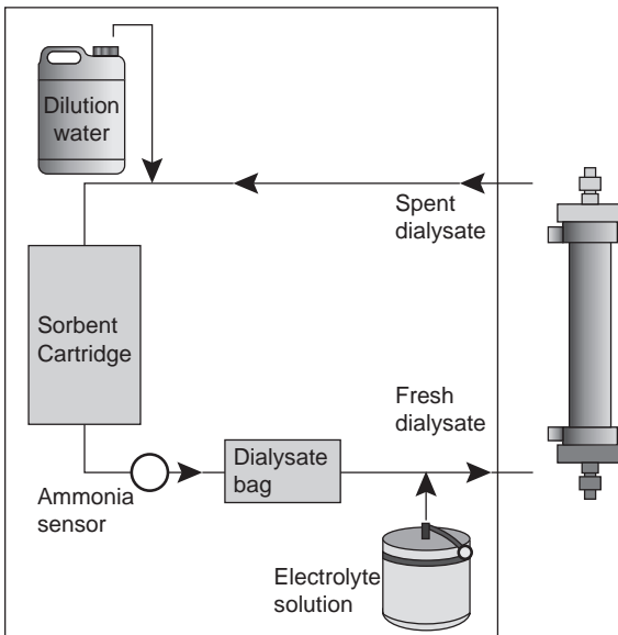
FIGURE 19.3 Schematic representation of dialysate flow path for the Fresenius portable sorbent system.
